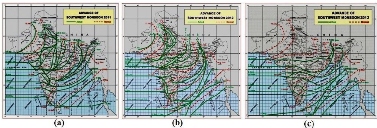
Fig. 4. Advance of SW monsoon for the years (a) 2011,(b) 2012 and (c) 2013 [www.imd.gov.in]
