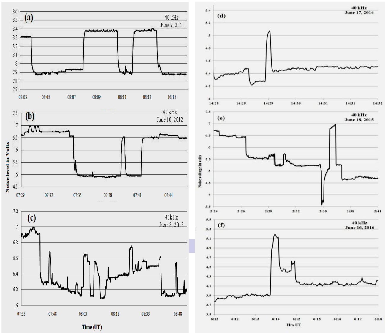
Fig. 2. Precursory effects in the atmospheric level before the arrival of SW monsoon at Kalyani, West Bengal
