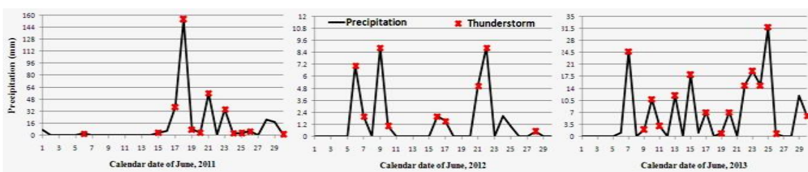
Fig. 6. (b) Precipitation with occurrence of thunderstorm for the month of June for three consecutive years
