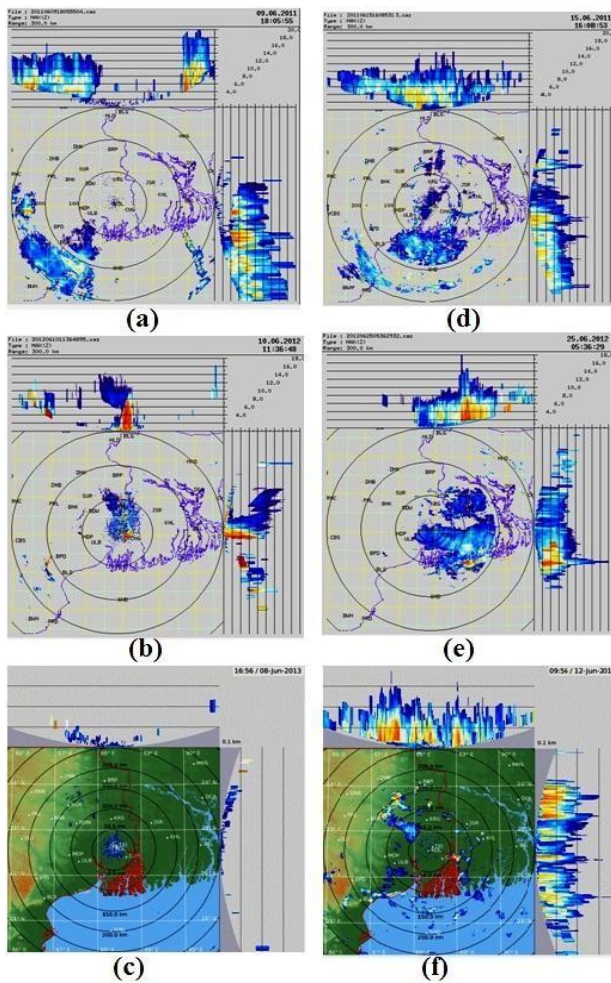
Fig. 9. Doppler Weather Radar pictures of some selected dates of interest as recorded at Kolkata observatory
