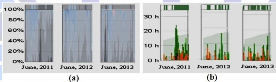
Fig. 5. (a) Cloud cover and (b) Precipitation for the month of June for three consecutive years
