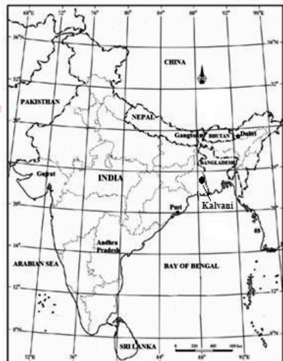
Fig.1. Map of India showing North and South Bengal including the locations of the Bay of Bengal and the location of Kalyani where atmospherics data were recorded
