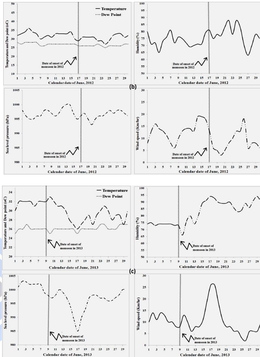
Fig. 8. Plots showing the variation of different atmospheric parameters before and after the monsoon onset for the years of (a) 2011, (b) 2012 and (c) 2013
