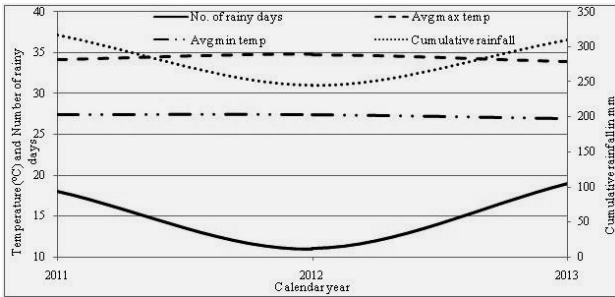
Fig. 7. Comparison of number of rainy days, average maximum temperature, average minimum temperature and cumulative rainfall for the first 19 days of monsoon for the three consecutive years
