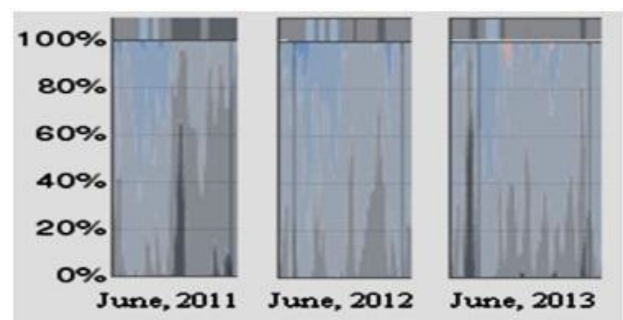
Fig. 6. (a) Cloud cover for the month of June for three consecutive years
